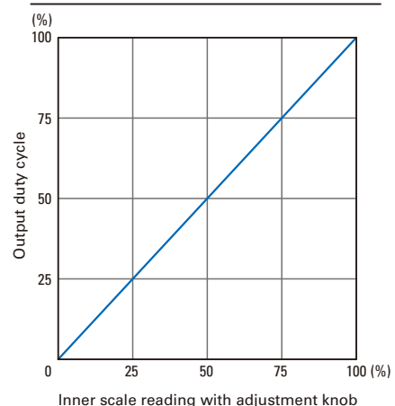
Inner Scale Reading - Output Duty Cycle Characteristics
