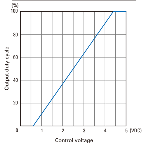
Control Voltage - Output Duty Cycle Characteristics
